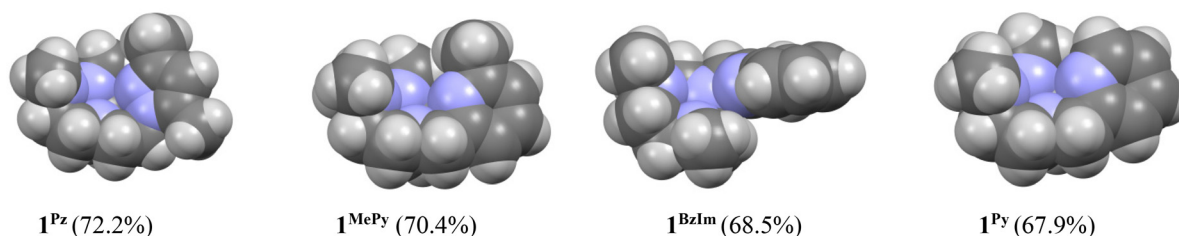
Fig. 8 Space filling models and the corresponding percent buried volume ( %V_{bur} ) values of the ligand pockets, within a 3.5 Å radius of the centrally located iron ion, in the Fe(II) precursor complexes 1Pz , 1MePy , 1BzIm and 1Py .
