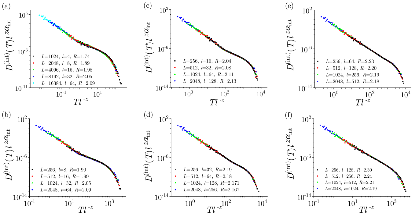
FIG. 8. Data collapsing of the integrated duration distributions D^{(\text{int})}(T) predicted by (C2). The range of l/L , and the values of disorder, are the same as in Fig. 7.
