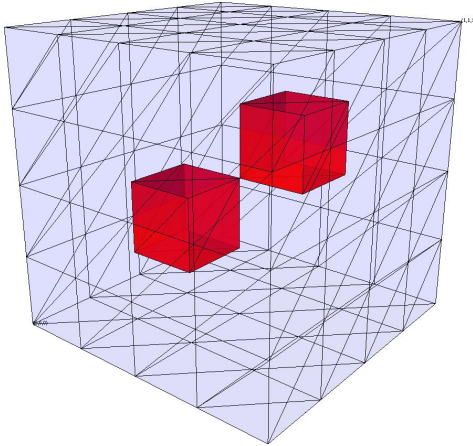
FIGURE 3. 3D Computational Domain
