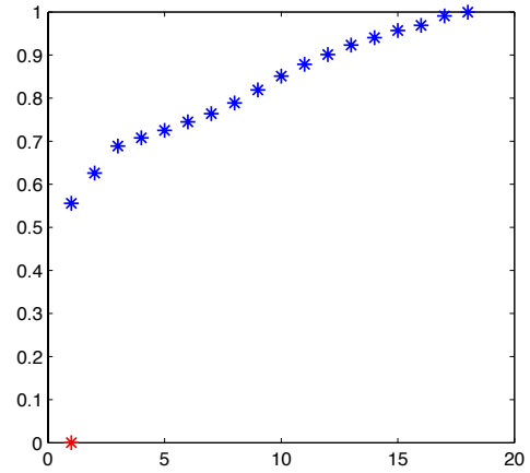
FIGURE 4. Eigenvalue Distribution of BA
