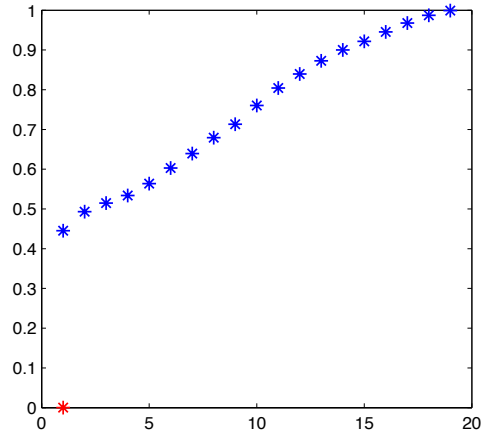
FIGURE 2. Eigenvalue Distribution of BA
