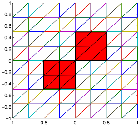
FIGURE 1. 2D Computational Domain
