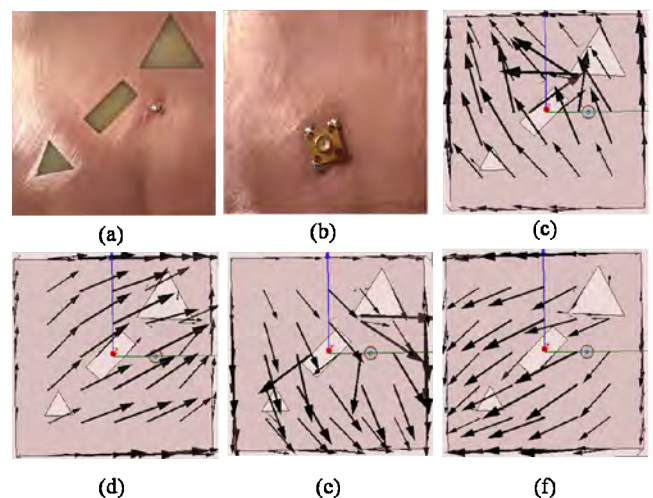
Fig. 3. (a)-(b) Fabricated prototype proposed antenna front view and back view and simulated surface current distribution at 910 MHz: (c) 0°, (d) 90°, (e) 180°, (f) 270°.
