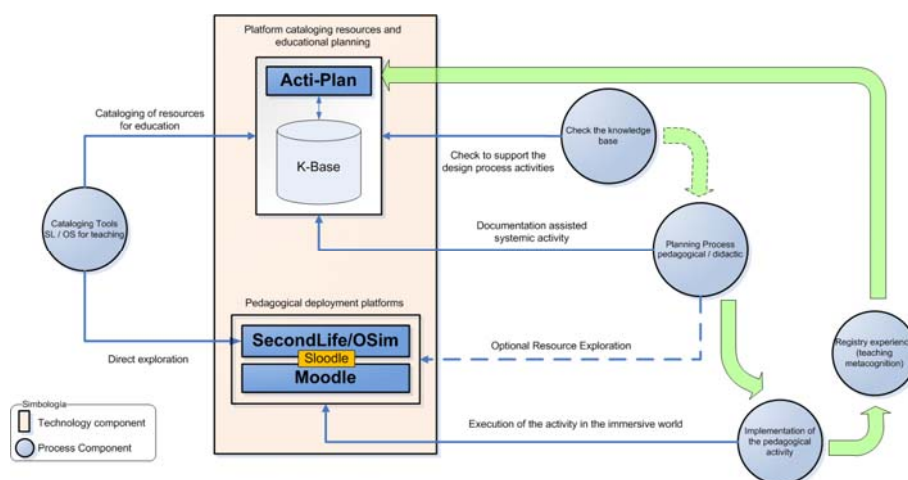
Figure 1: A technological model for teaching in Immersive Worlds: TYMMI Project [Badilla & Lara, 13]
