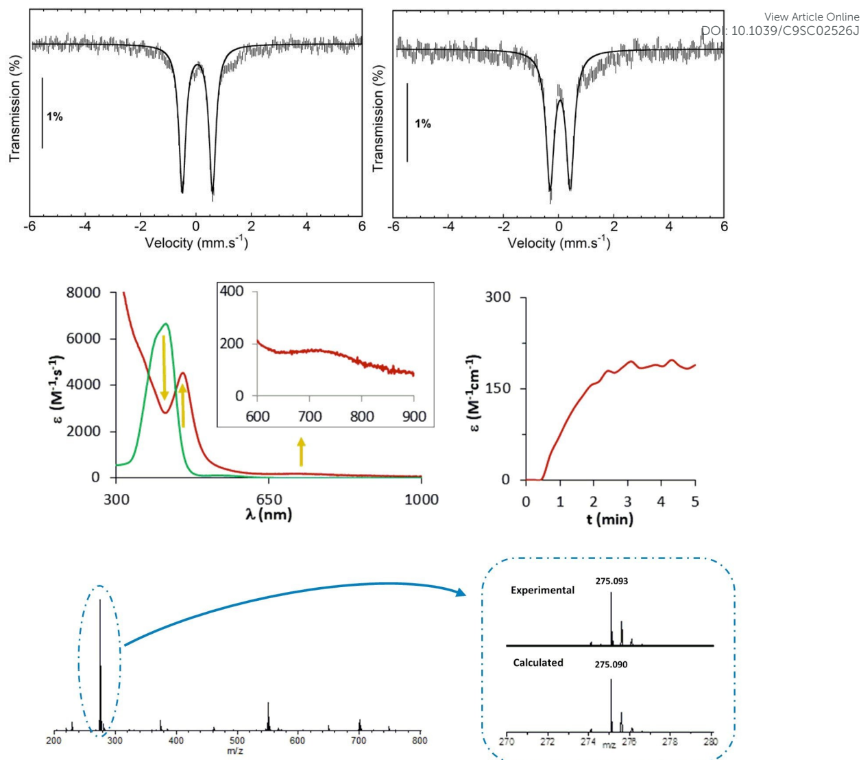
Figure 1. Top, Mössbauer spectrum recorded at 80 K in zero-field of 1 (IV) =NTs (left) in acetonitrile and 2 (IV) =NTs (right) prepared in acetone. Experimental data are hatched bars and solid lines represent the contributions of 1 (IV) =NTs and 2 (IV) =NTs. Centre, UV-vis spectrum of oxidation of 1 (II) to 1 (IV) =NTs in CH 3 CN; kinetic trace shows the evolution of the λ max = 750 nm feature. Below, HR-MS spectrum of 1 (IV) =NTs prepared in CH 3 CN exhibiting a base peak at m/z 275.09; inset show amplification of major peak for [Fe IV (NTs)(MePy 2 tacn)] 2+ species. Proper simulation of the peak requires inclusion of ≈10 % of [Fe III (NHTs)(MePy 2 tacn)] 2+ in the isotopic pattern corresponding to [Fe IV (NTs)(MePy 2 tacn)] 2+ .
