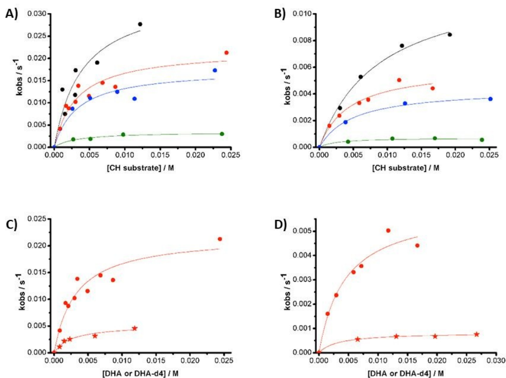
Figure 10. Observed reaction rates ( k_{obs} ) derived from the reaction of a) 1^{(IV)}=NTs and b) 2^{(IV)}=NTs against different substrates in acetonitrile solution at 293 K under N_2 . Substrates: Black = xanthene; red = DHA; blue = CHD; green = fluorene. c) 1^{(IV)}=NTs and d) 2^{(IV)}=NTs against DHA (circles) and DHA-d 4 (stars).
