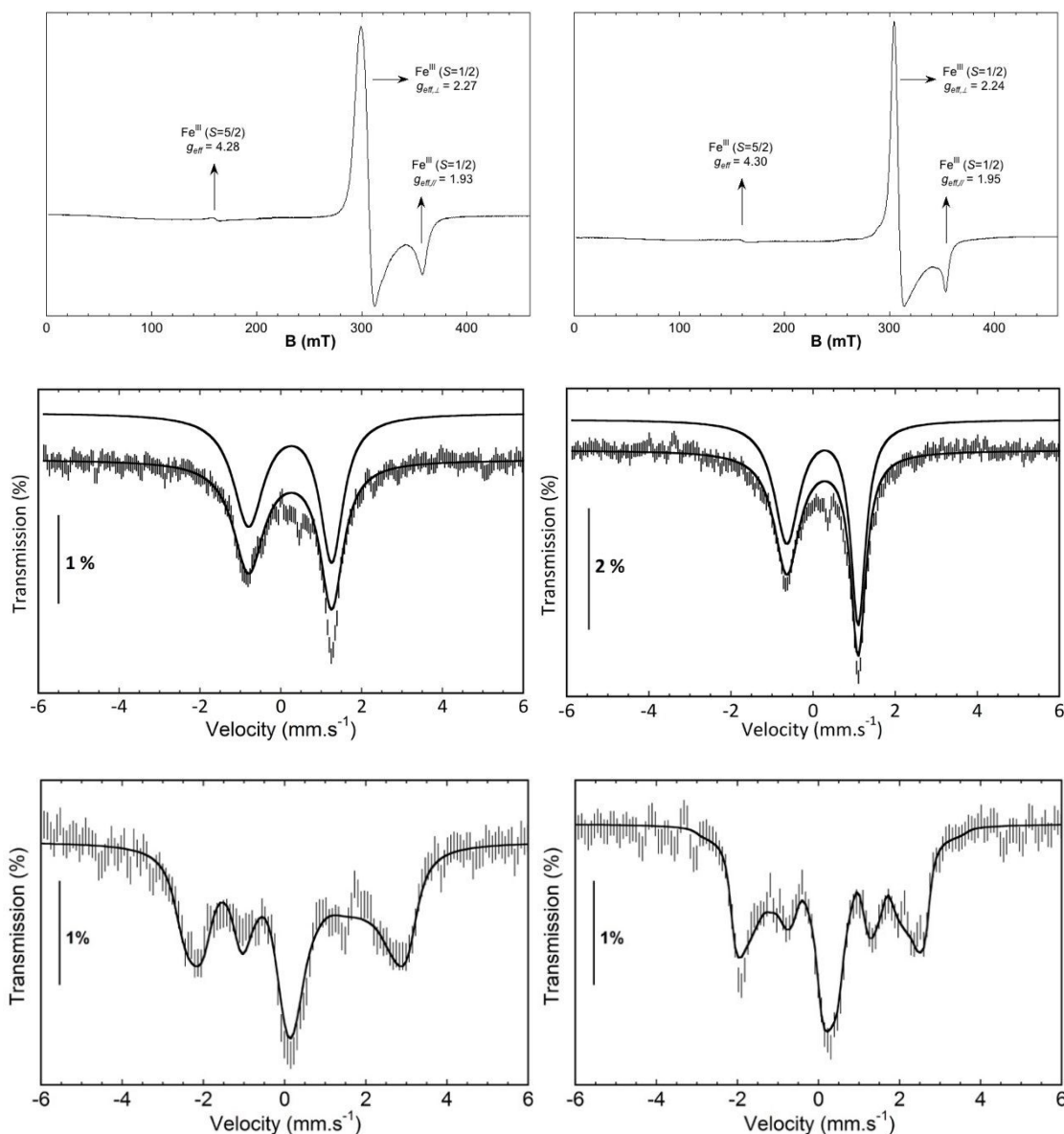
Figure 7. Spectroscopic data of isolated 1 (III) -NHTs (left) and 2 (III) -NHTs (right). (Top) EPR spectra of 1 (III) -NHTs (left) and 2 (III) -NHTs (right). Middle, Mössbauer spectra of 1 (III) -NHTs (left) and 2 (III) -NHTs (right) recorded at 80 K in absence of field (middle) and at 4.2 K under a field of
