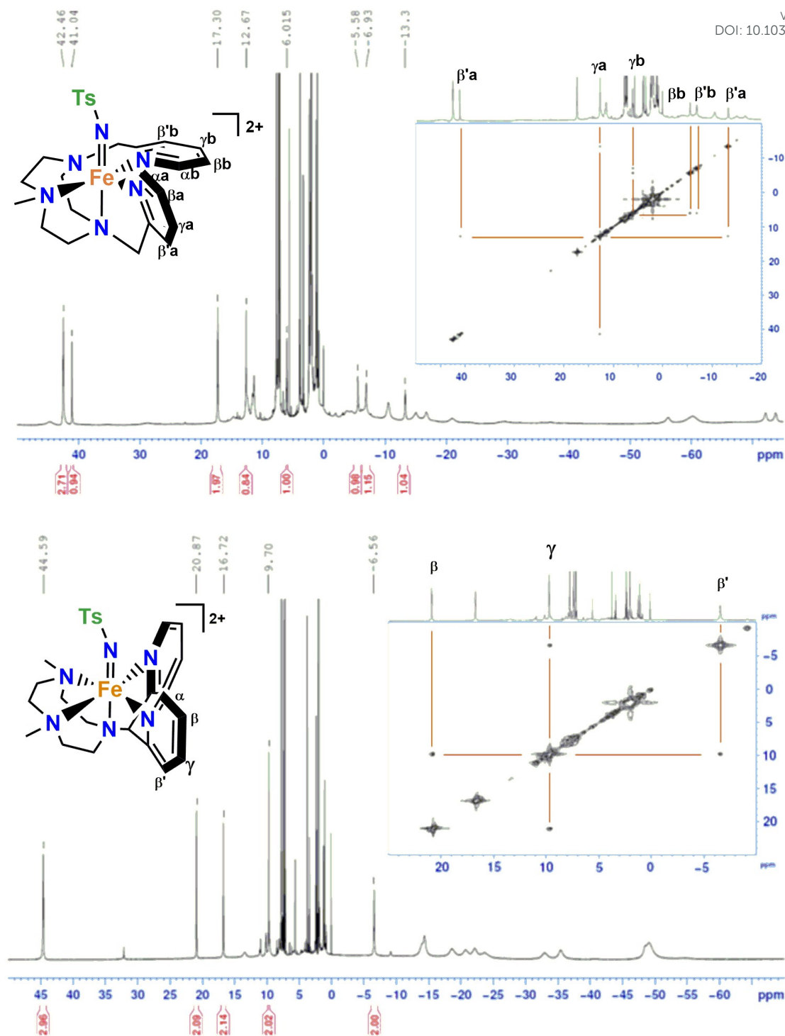
Figure 2. ^1\text{H} -NMR and COSY spectra of 1^{(\text{IV})}=\text{NTs} (top) in acetone- d_6 at 0^\circ\text{C} and 2^{(\text{IV})}=\text{NTs} (bottom) in acetone- d_6 at 25^\circ\text{C} ; small peaks at 32 and -9 ppm belong to <5\% of 2^{(\text{IV})}=\text{O} .
