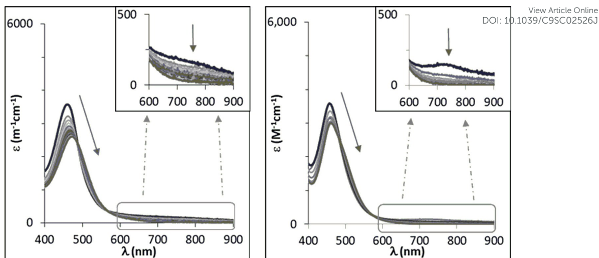
Figure 8. UV – vis spectra corresponding to the reaction of 1^{(IV)}=NTs (left) and 2^{(IV)}=NTs (right) upon addition of an excess of MeOPhSMe (reaction at 20 °C with 100 and 50 eq of substrate added respectively, [Fe] = 0.25 mM in MeCN). Spectra correspond to the first rapid phase of the reaction.
