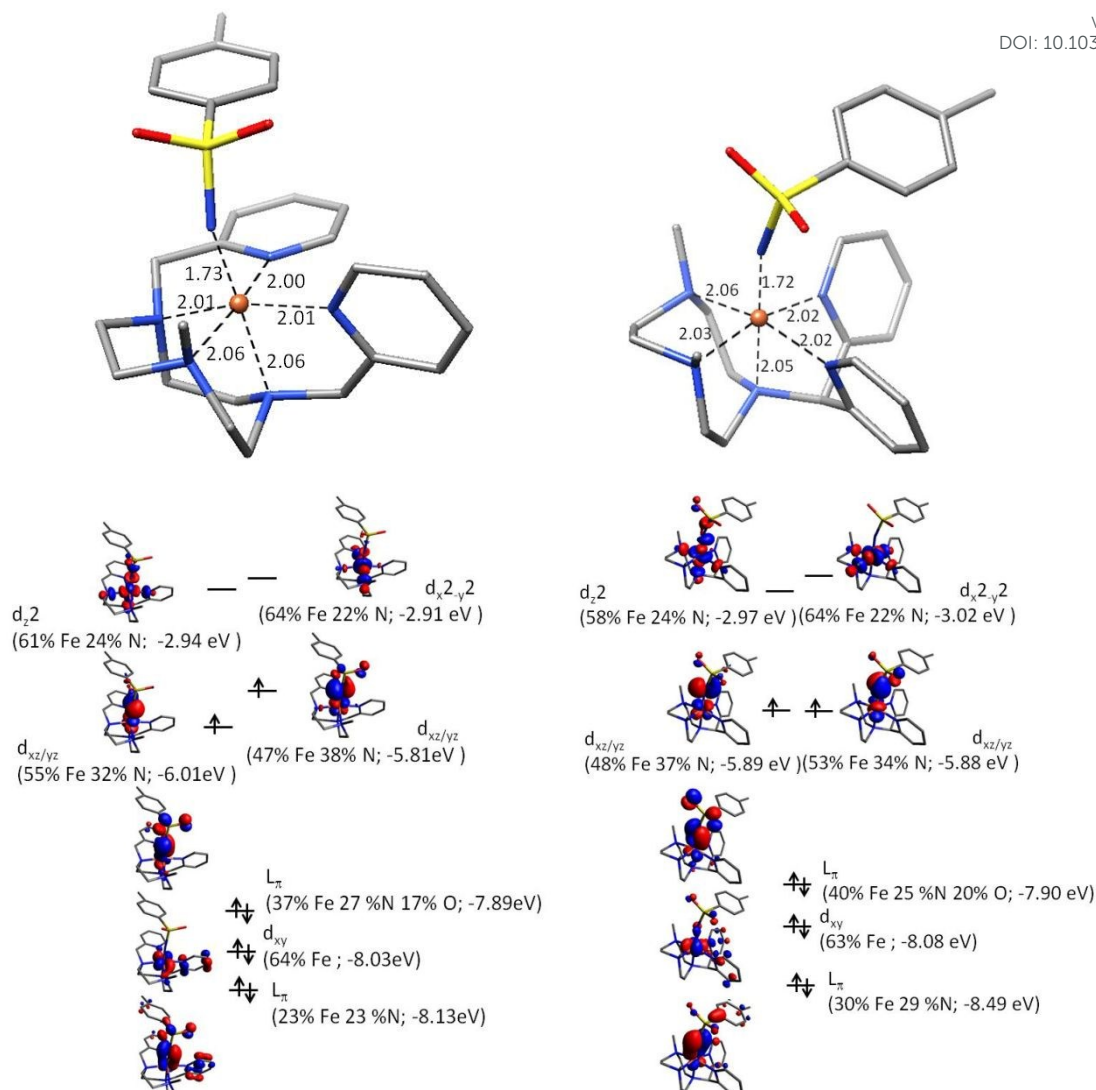
Figure 5. (top) Computationally derived geometries showing first coordination shell bond distances. (Bottom) Schematic of Fe=NTs molecular orbitals showing the iron d – manifold using quasi – restricted orbitals (0.05 isovalue) for 1^{(IV)}=NTs (left) and 2^{(IV)}=NTs (right).
