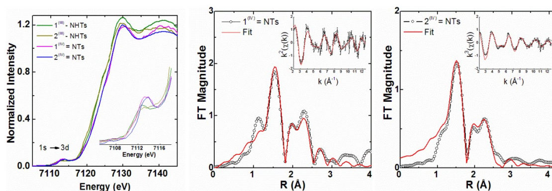
Figure 4. Iron K-edge XANES region (left) for 1^{(III)}-NHTs , 2^{(III)}-NHTs , 1^{(IV)}=NTs and 2^{(IV)}=NTs together with (right) non – phase shift corrected Fourier transforms of EXAFS data for 1^{(IV)}=NTs and 2^{(IV)}=NTs with insets showing the k – space data and fits. Experimental data are shown in black and fits in red (see fit tables S4-S7).
