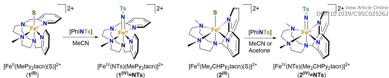
Scheme 1. Chemical strategy for the generation of 1^{(IV)=NTs} and 2^{(IV)=NTs} from iron (II) precursors. 1^{(II)} and 2^{(II)} (S = MeCN, CF_3SO_3 ).
