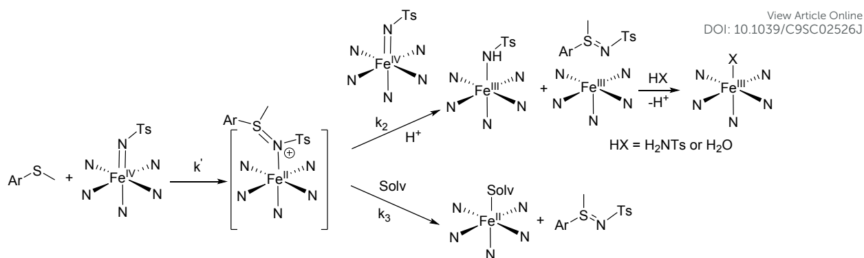
Scheme 3. Mechanism proposal for the first phase of the reactions of iron (IV) – tosylimido complexes with thioanisole substrates. Solv. stands for solvent molecule.
