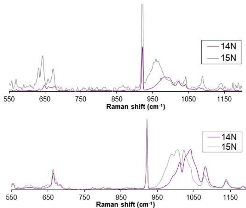
Figure 3. Resonance enhanced Raman spectra for complex 1^{(IV)}=NTs (top) and 2^{(IV)}=NTs (bottom) upon excitation at 488 nm.
