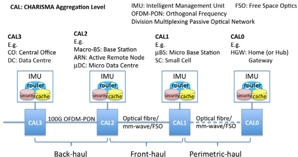
Figure 2: Hierarchical CHARISMA Aggregation Levels (CALs)
