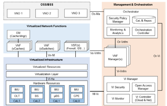
Figure 4: High-level CHARISMA control, management, and orchestration plane
