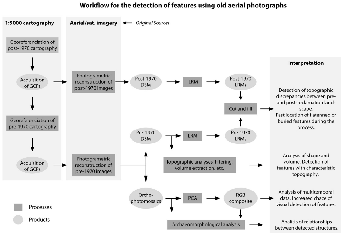
Fig. 5. Scheme of the workflow followed for the photogrammetric-based multi-temporal Remote Sensing (RS) analysis of the study area.
