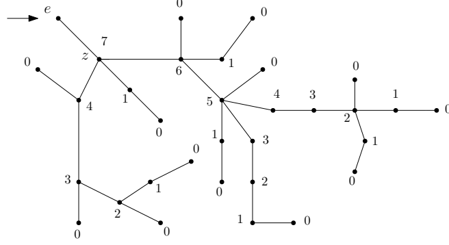
FIGURE 9. Topological induction
