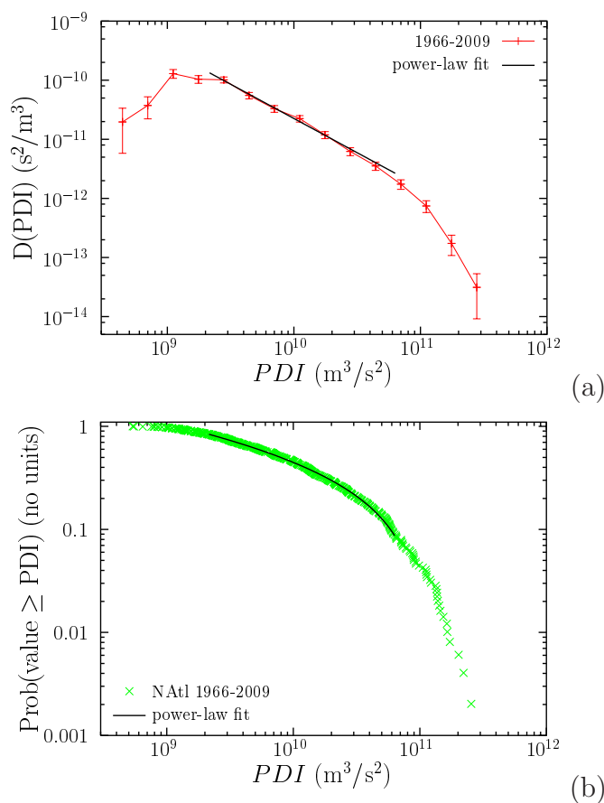
FIGURE 3. (a) Empirical probability density of 1966-2009 North-Atlantic individual tropical-cyclone PDI (494 events), together with a power-law fit between 2.2 \cdot 10^9 and 6.3 \cdot 10^{10} \text{m}^3/\text{s}^2 with an exponent \tau = 1.16 . See Corral et al. (2010). (b) Same data and fit as in the previous panel but for the (complement of the) cumulative distribution function. Notice that the power-law distribution is no longer a straight line in a log-log plot, due to the bending effect of the upper truncation, which adds a constant to the power law ?. In this plot, the KS distance turns out to be proportional to the maximum difference between the empirical cumulative density and its fit (rather small).
