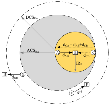
Fig. 1: Appropriate carrier sensing range that just covers the interference range.
