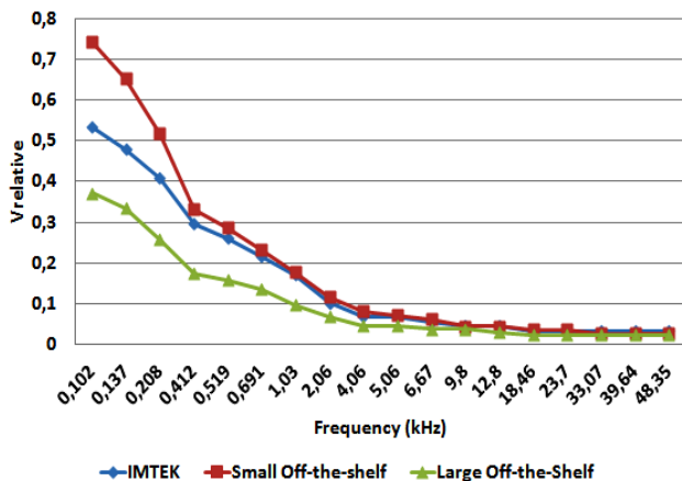
Fig. 3. Indoor solar panel responses to different frequencies.
