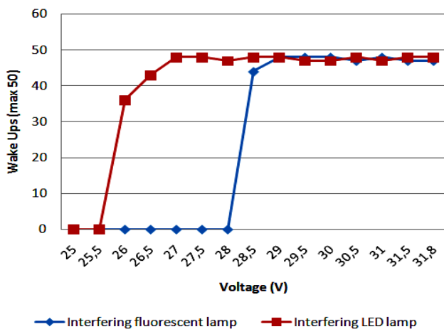
Fig. 7. Number of wake-ups generated for different LED voltage levels with interference from other light sources.
