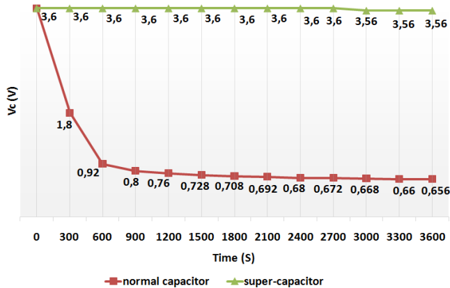
Fig. 4. Leakage test results for the electrolytic capacitor of 470\mu\text{F} and super-capacitor of 1\text{F} .
