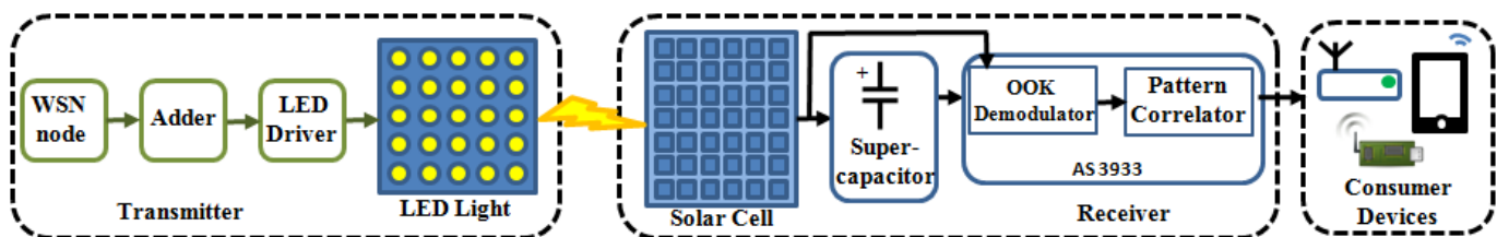
Fig. 1. Global system view of the energy-autonomous VLC wake-up system.
