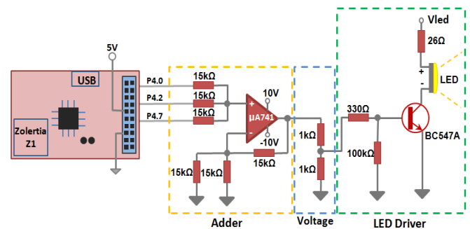
Fig. 5. Transmitter circuit diagram.
