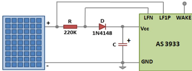
Fig. 2. Circuit diagram of the wake-up receiver.
