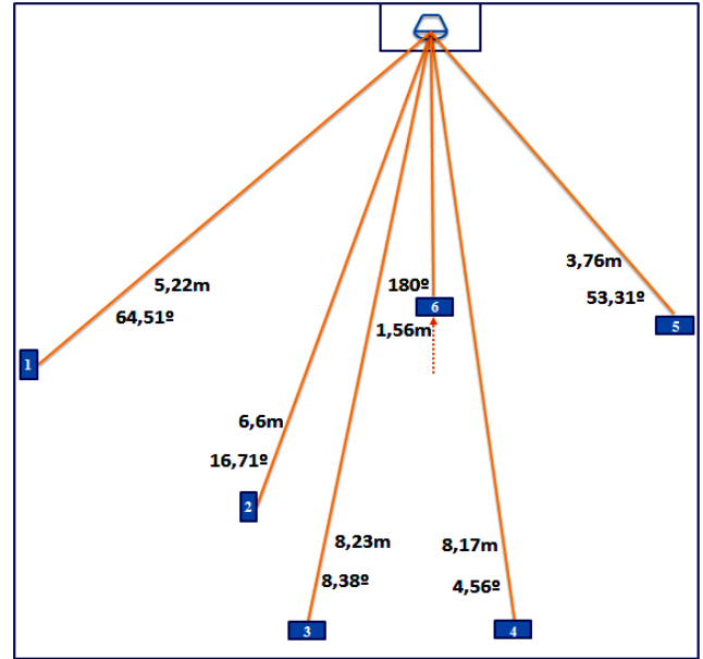
Fig. 6. Positions (distance and angles) tested with high probability of detecting wake-up frames.
